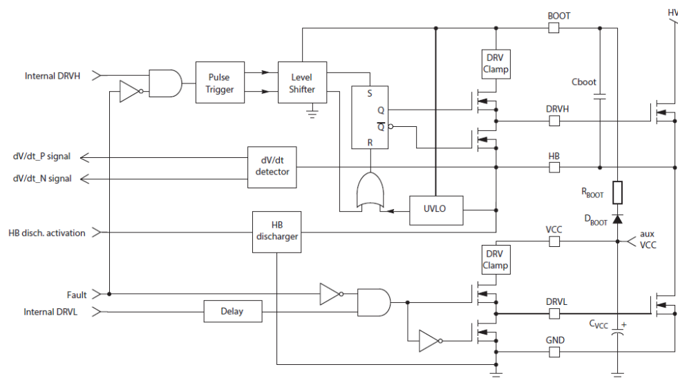
Figure 65. The NCL30159 Internal DRVs Structure
