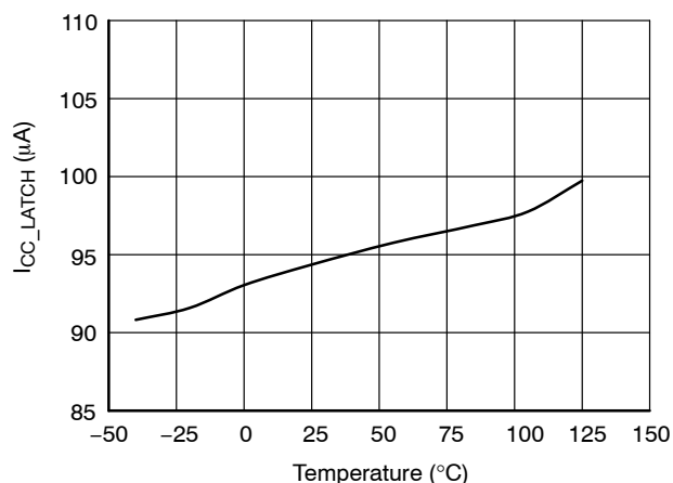
Figure 23. Internal Current Consumption in Fault Mode (Latch) I_{CC\_LATCH}
