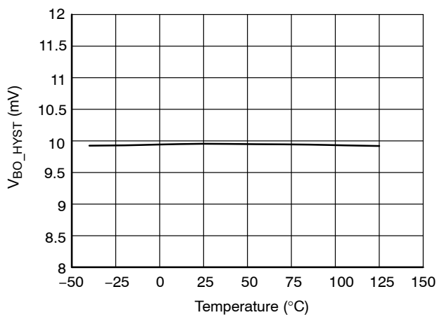
Figure 38. Brown-out Comparator Hysteresis V_{BO\_HYST}
