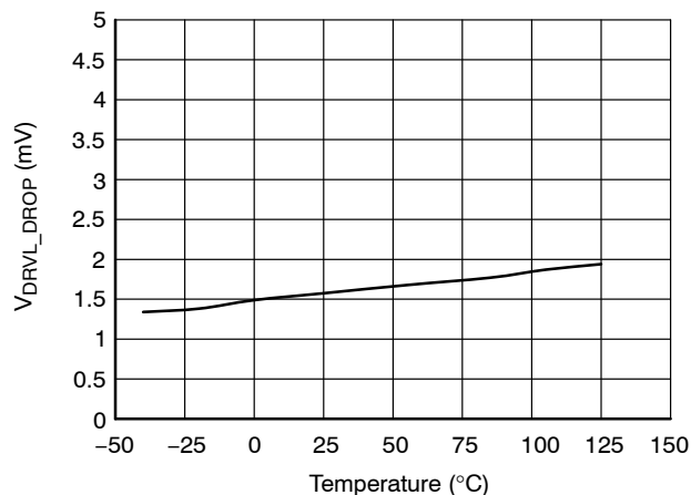
Figure 32. Low Side Driver Voltage Drop VDRV_L_DROP
