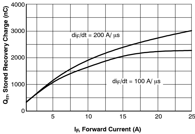
Figure 20. Stored Charge
