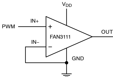
Figure 39. Dual-Input Driver Enabled, Non-Inverting Configuration
