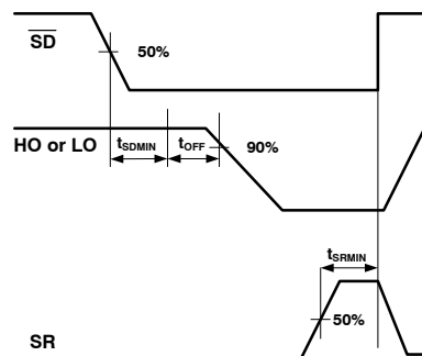
Figure 36. Shutdown with SR Pin Pulled Down – Timing Waveform Definition
