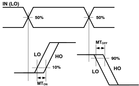
Figure 34. Delay Matching Waveform Definition
