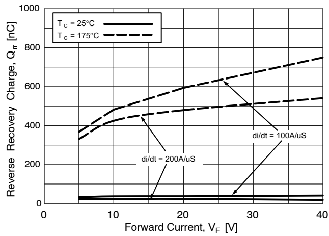
Figure 19. Stored Charge
