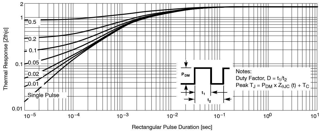
Figure 21. Transient Thermal Impedance of Diode
