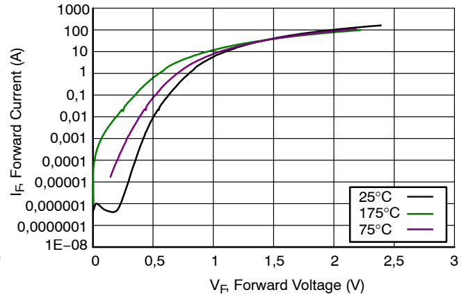
Figure 16. Forward Characteristics
