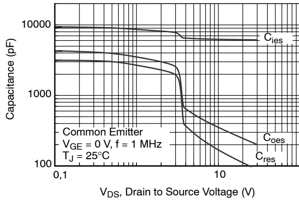
Figure 7. Capacitance Characteristics
