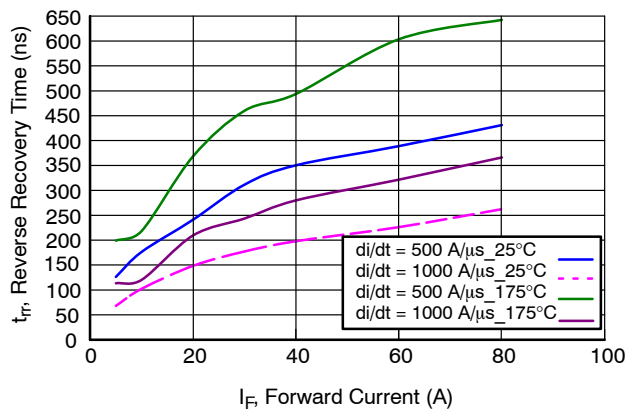
Figure 17. Reverse Recovery Time
